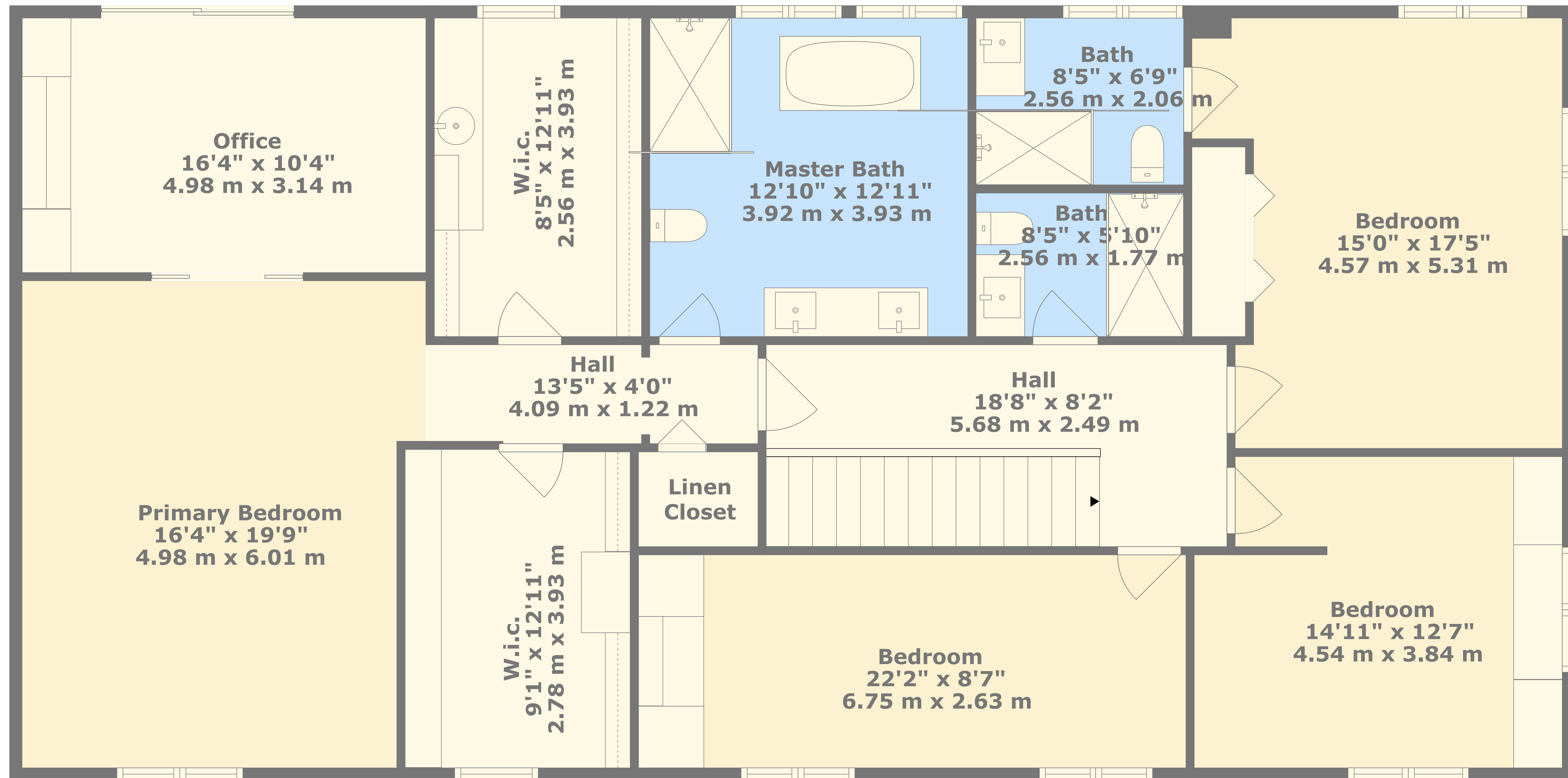
Floor 2
